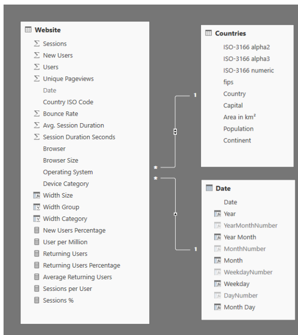
Figure 7-29: A schema of tables and relationships of a data model that extends Google Analytics website data.
