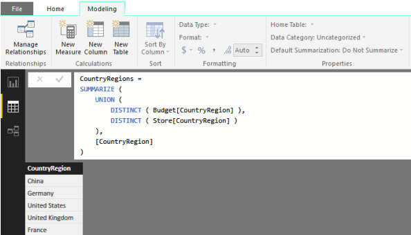
Figure 6-11: You can populate a calculated table with the distinct values of CountryRegion.
