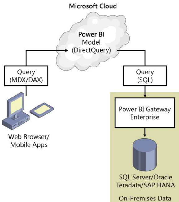
Figure 8-2: For on-premises data sources, you must have the Power BI Enterprise Gateway for a model using the DirectQuery connection setting.
