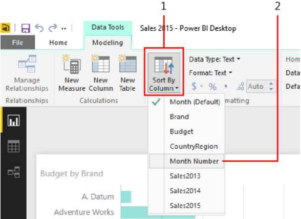
Figure 4-27: You can sort month names by numbers by using the Sort By Column feature.
