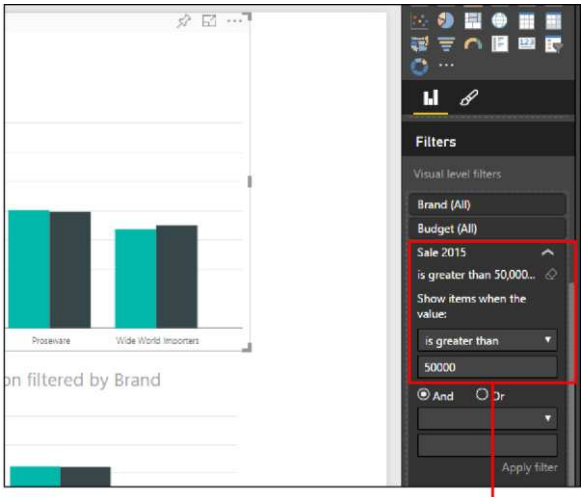
Visual-level filters
