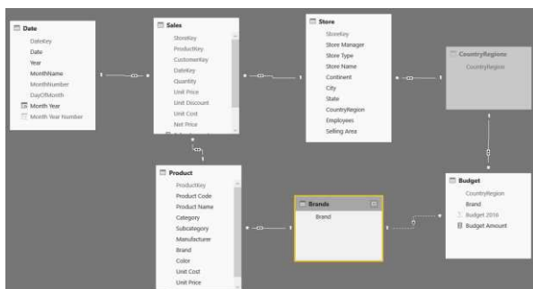
Figure 6-15: Among the many relationships, the one between Brands and Budget is inactive, signified by the dashed connector line between them.
