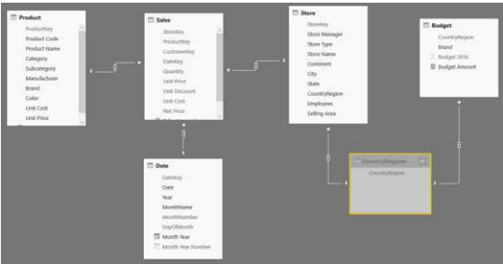
Figure 6-12: The CountryRegions table acts as an intermediate between Store and Budget.
